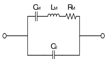
Fig.1 RF Equivalent RLC Model
