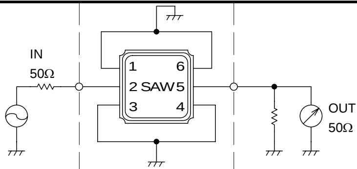
Fig.1 Measuring circuit
